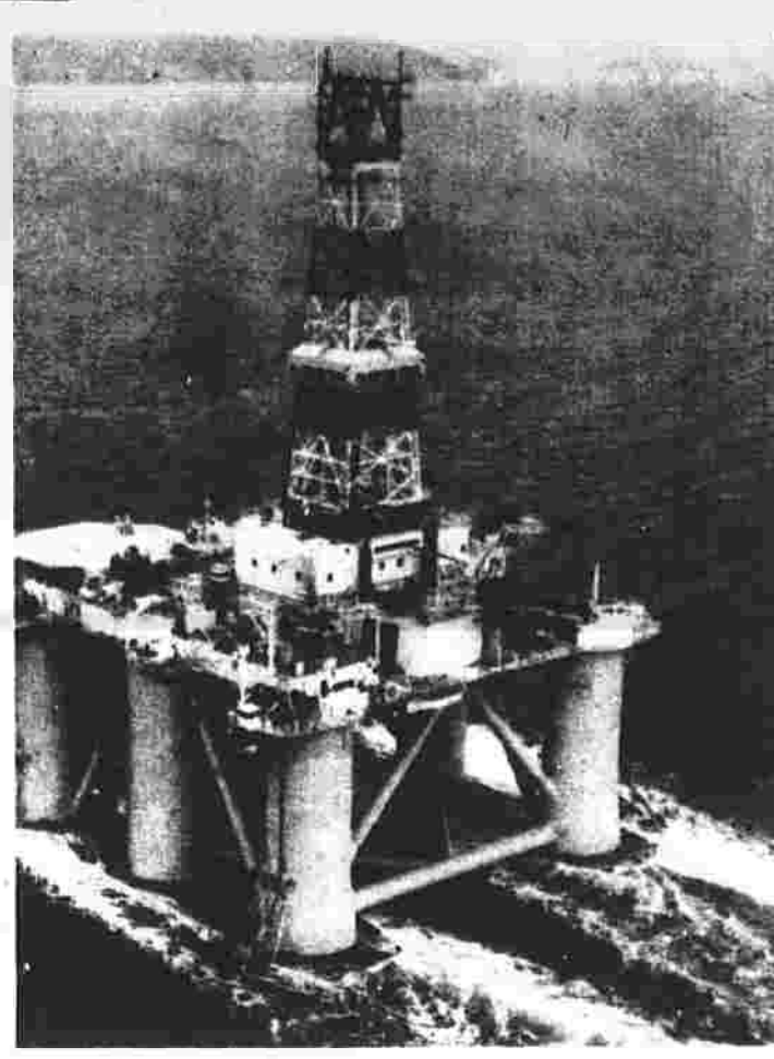
This drilling rig called the Alaskan Star, now in use in the Baltimore Canyon area of the Mid-Atlantic will be used by Exxon Company USA to begin exploration in the Georges Bank area of the North Atlantic in August. The semi-submersible drilling vessel is designed for severe sea conditions and sub-arctic temperatures. (UPI photo)
